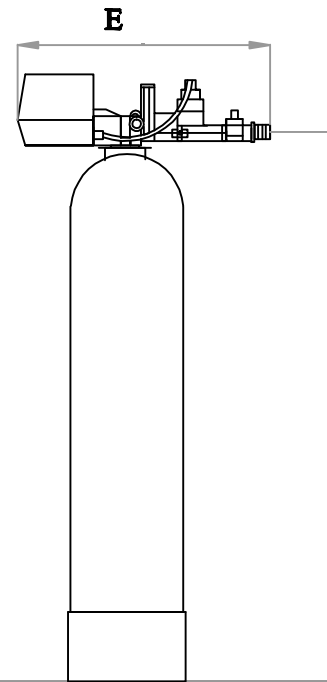
SIDE VIEW - MINERAL TANK
