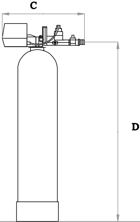
SIDE VIEW -MINERAL TANK
